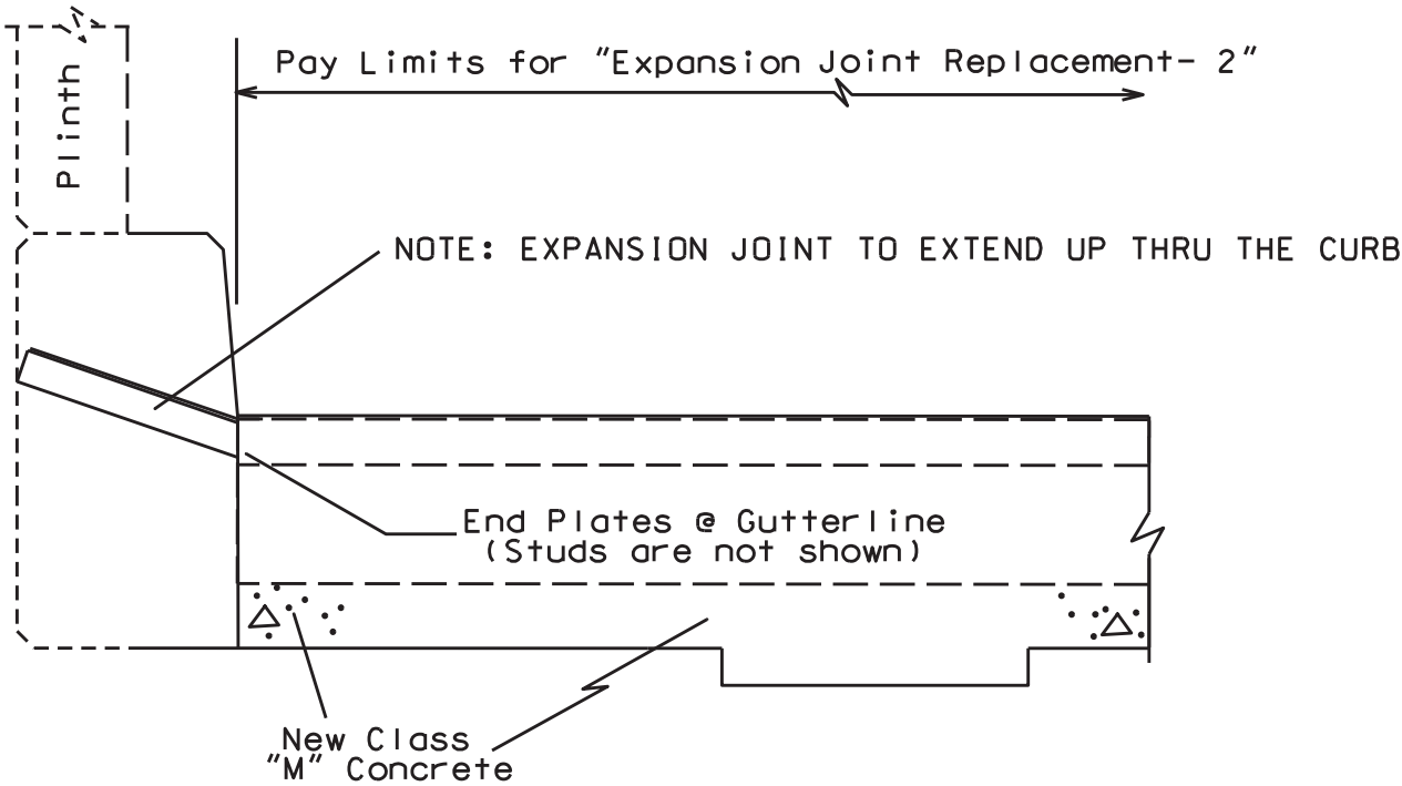
PROPOSED SECTION @ CURB
